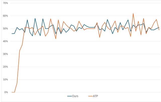
Figure 4. PQ Hit Ratio comparison after a context switch .
